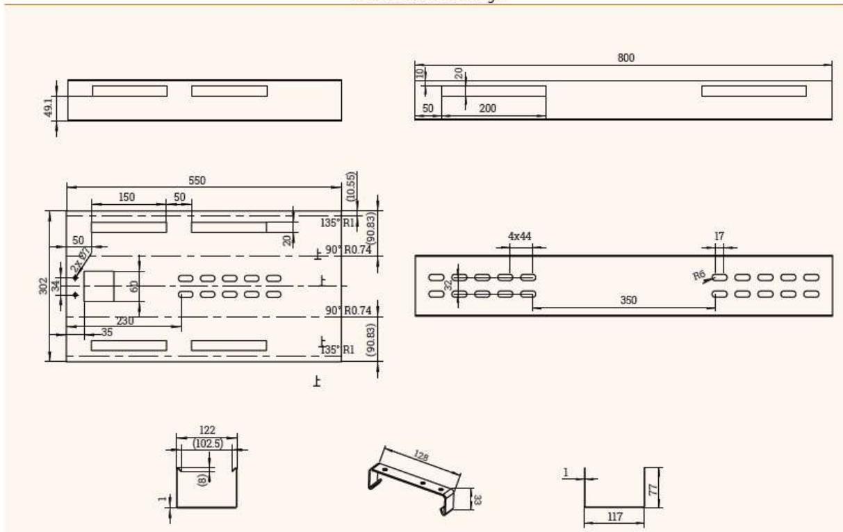
Technical Drawings
